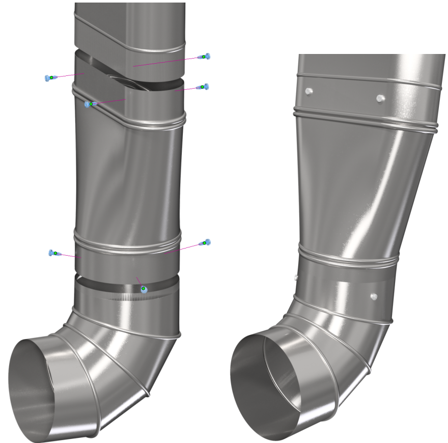
INSTALLED VIEW
