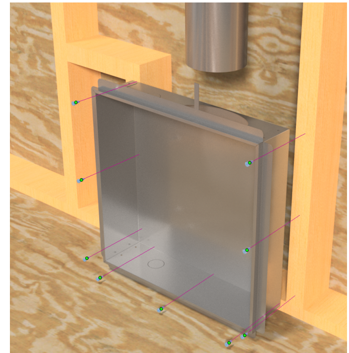
INSTALLATION VIEW
