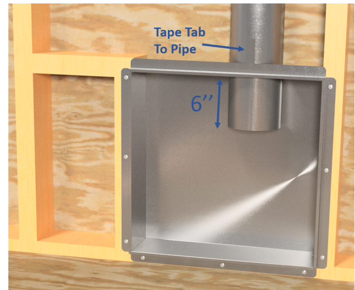
INSTALLED VIEW
